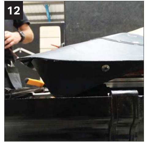
12 The hip tile is closed off by the end stop.
